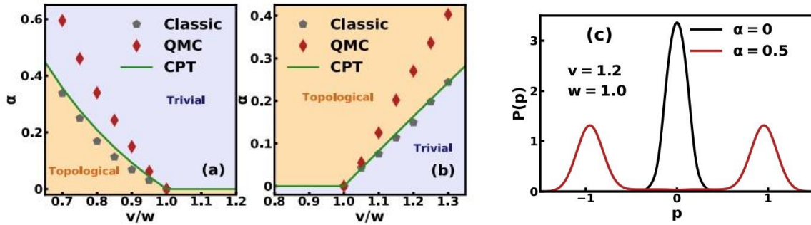
Fig. 1 . Phase diagram, in the case of intra[inter]cell hopping coupled with local baths in (a) [(b)], for quantum (red diamonds) and classical bosons (grey points) through MC technique. Green line denotes the critical values of the couplings obtained through CPT for quantum baths. (c) Polarization probability distribution in the case of intercell hopping coupled with local baths.
